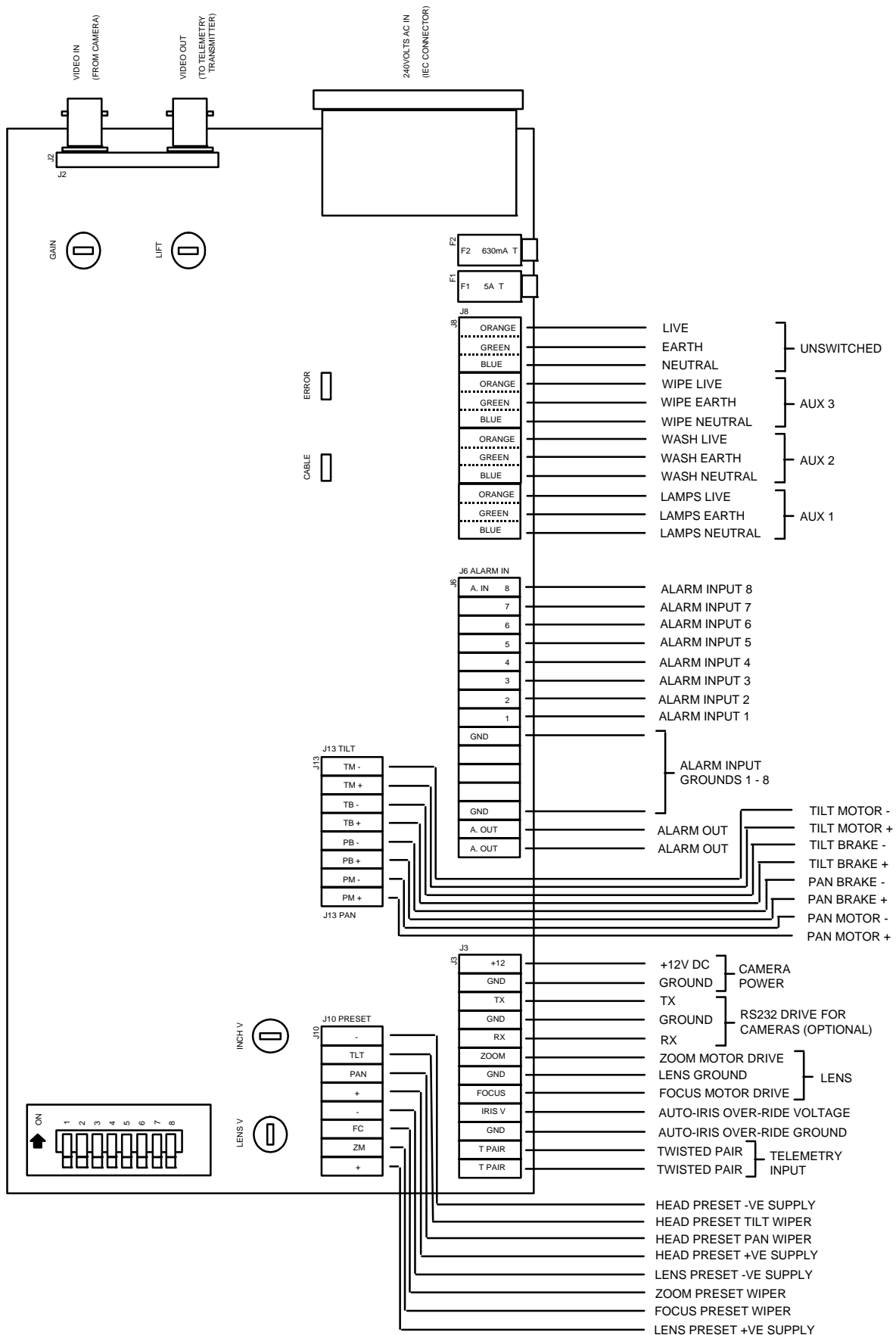
Fig. 2: Cable connection diagram
