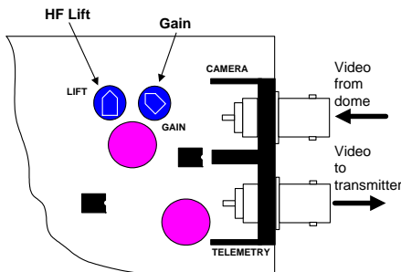
Fig. 4 Launch Amplifier
