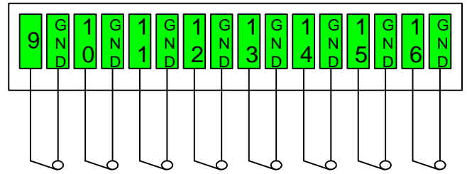
Each input has 56K internal pull up to 9Vdc
