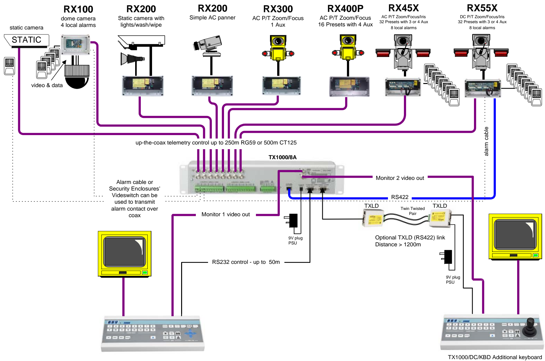
A Simple TX1000 System
